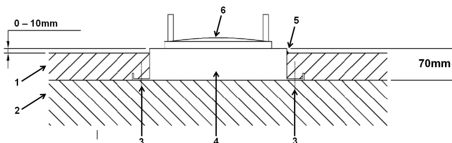
Fig. 0-13 Fixture sideview
