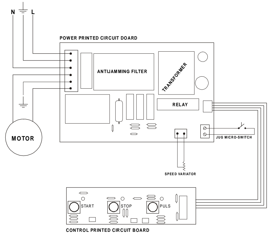
FIG. n°6 - Wiring diagram Mn - Orione in aluminium
