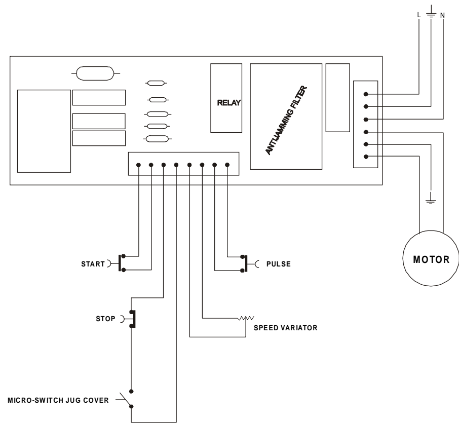
FIG. n°5 - Wiring diagram Mn - Orione in steel
