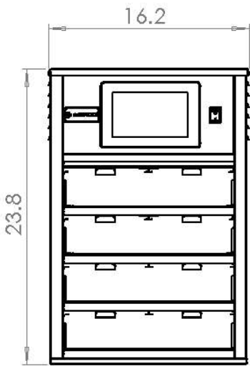
Front View: Model MHD42SSL1W
